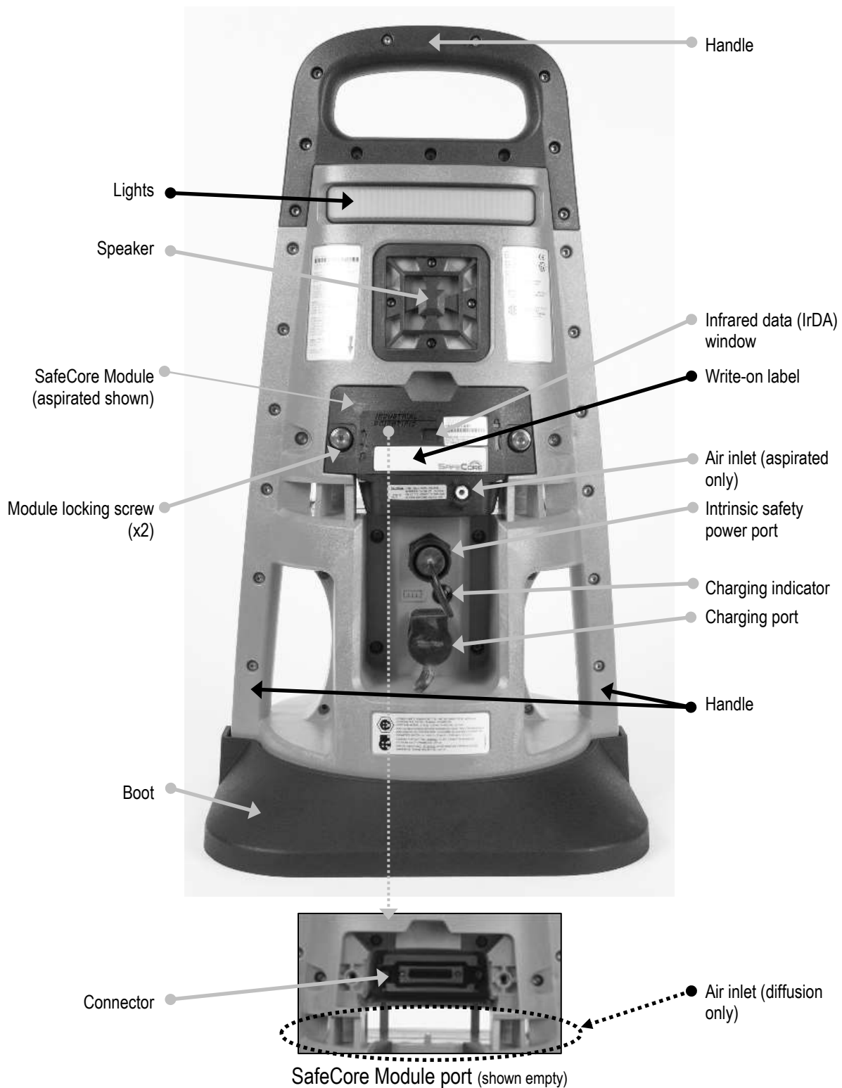
Figure 3.1.B Hardware overview Radius BZ1 (back view; aspirated)
