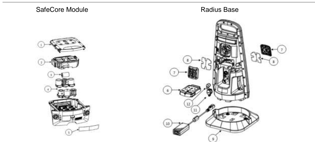
Figure 8.1 Parts diagram for SafeCore Module and Radius Base
