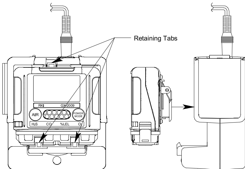
Figure 15 : Putting the GX-2009 in the Charging Base
