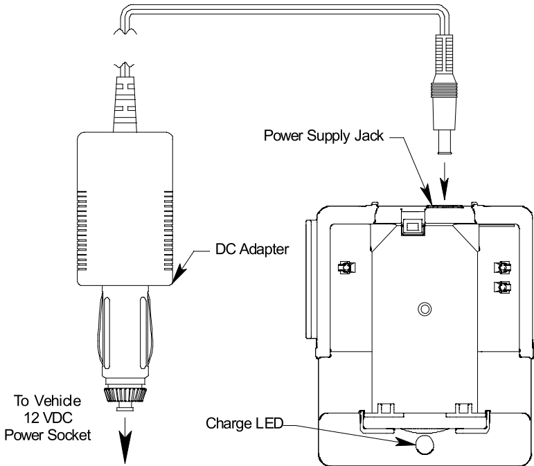
DC Powered Charging Station
