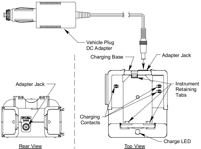
Figure 7 : GX-2009 DC Powered Charging Station
