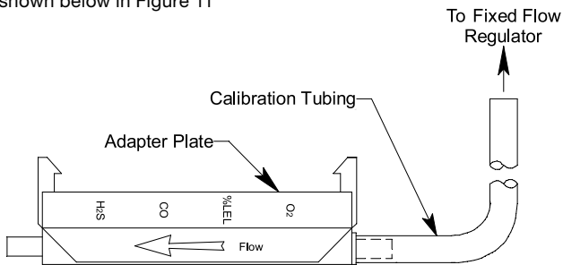
Figure 11 : Calibration Kit Assembly
