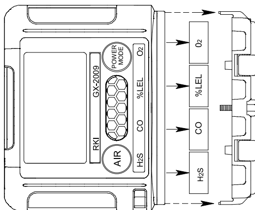
Figure 22 : Removing the Sensor Retainer to Replacing Sensor
