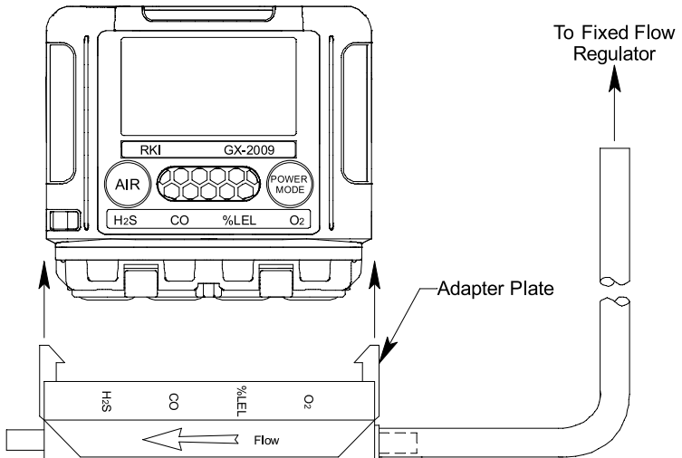
Figure 10 : Installing the Adapter Plate, Auto Cal
