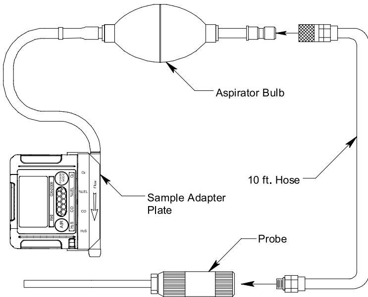
Figure 8 : GX-2009 Aspirator Adapter
