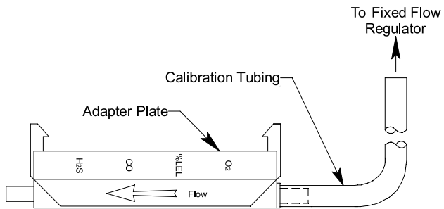
Figure 9 : Calibration Kit Assembly
