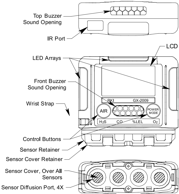
Figure 1 : GX-2009, Front & Bottom View
