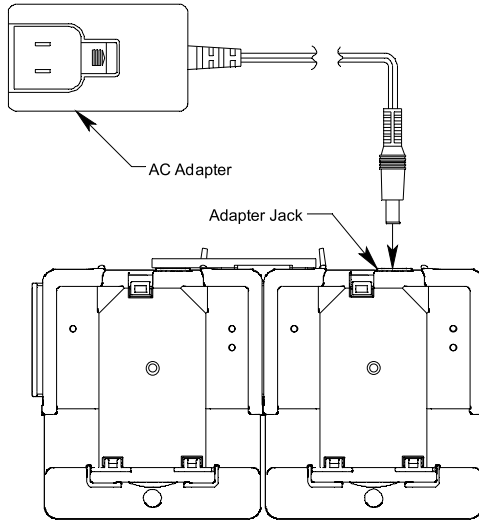
Figure 5 : GX-2009 Charging Station, Two Instrument Station
