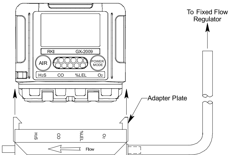
Figure 12 : Installing the Adapter Plate, One Cal
