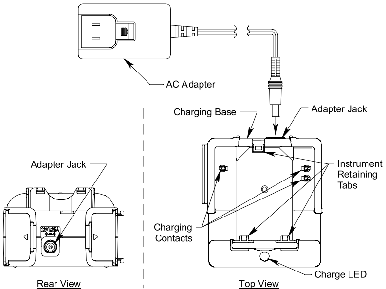
Figure 4 : GX-2009 Charging Station, Single Instrument Station
