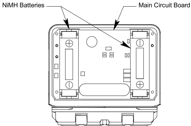
Figure 19 : NiMH Batteries
