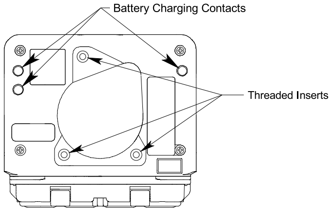
Figure 2 : GX-2009 Rear View
