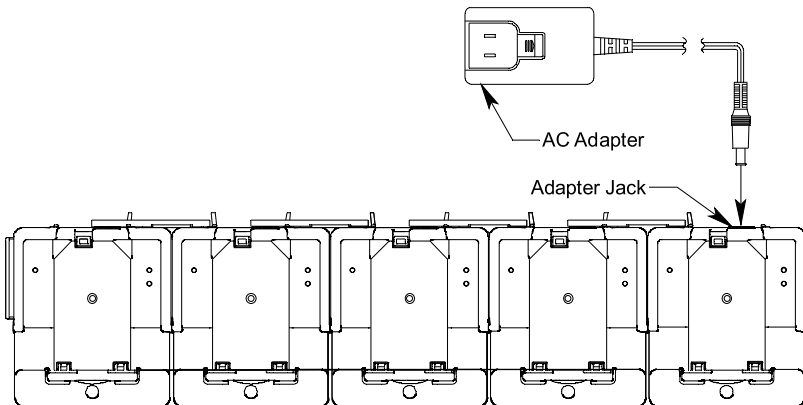
Figure 6 : GX-2009 Charging Station, Five Instrument Station
