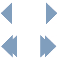
Figure 12: Home screen
